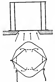
Figs. 4323-24, DOUBLE-DUPLEX DEFLECTOR (VERTICAL).
